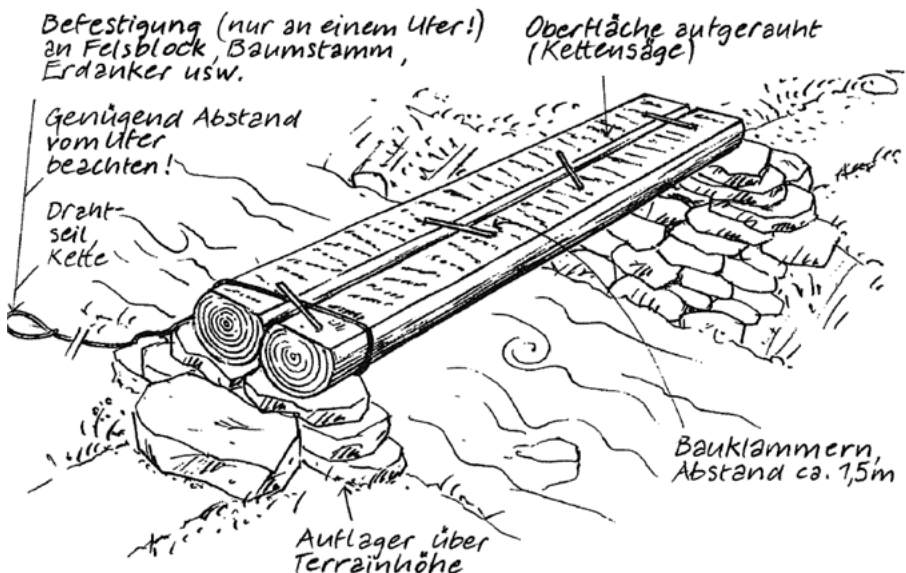
Abb. 85: Rundholzsteg (ASTRA)
